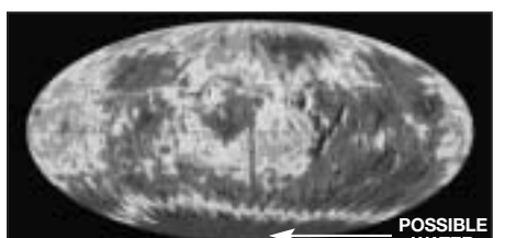
This Odyssey view of Mars shows big areas of hydrogen in the bottom area.
