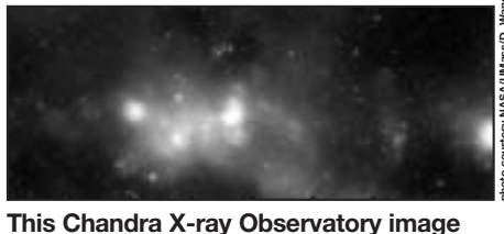
This Chandra X-ray Observatory image shows the central region of our Milky Way galaxy. In it are hundreds of white dwarf stars and black holes. Colorful gas heated to millions of degrees surrounds the stars.
